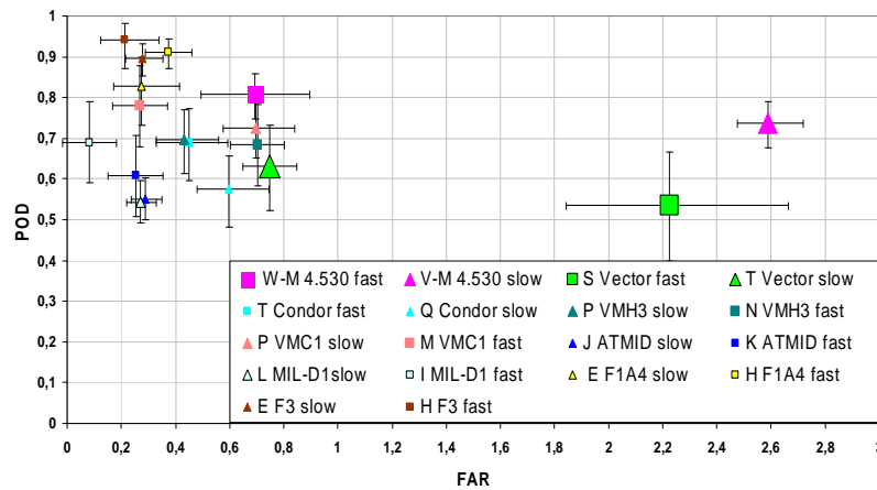
Figure 39: ROC diagrams of slowest and fastest operators
