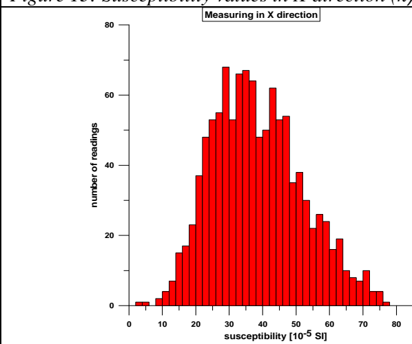
Figure 13: Susceptibility values in X-direction ( \kappa )
