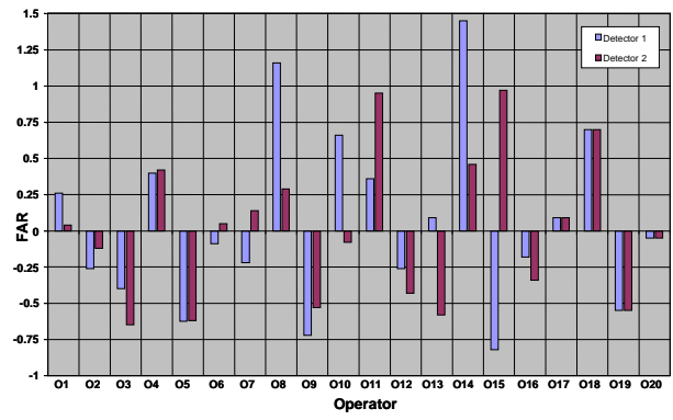
Figure 45. FAR coefficients for all operators and both detectors
